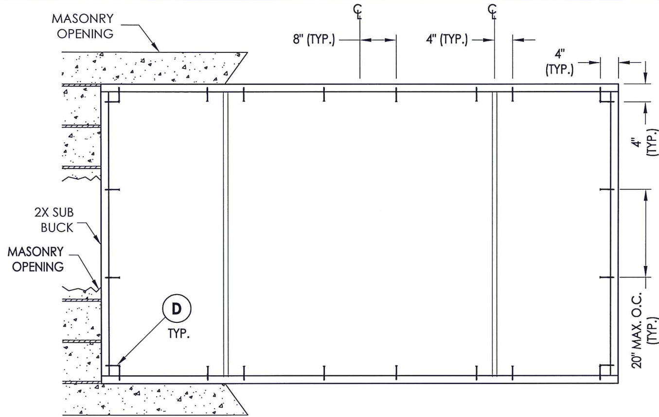
BUCK ANCHORING
