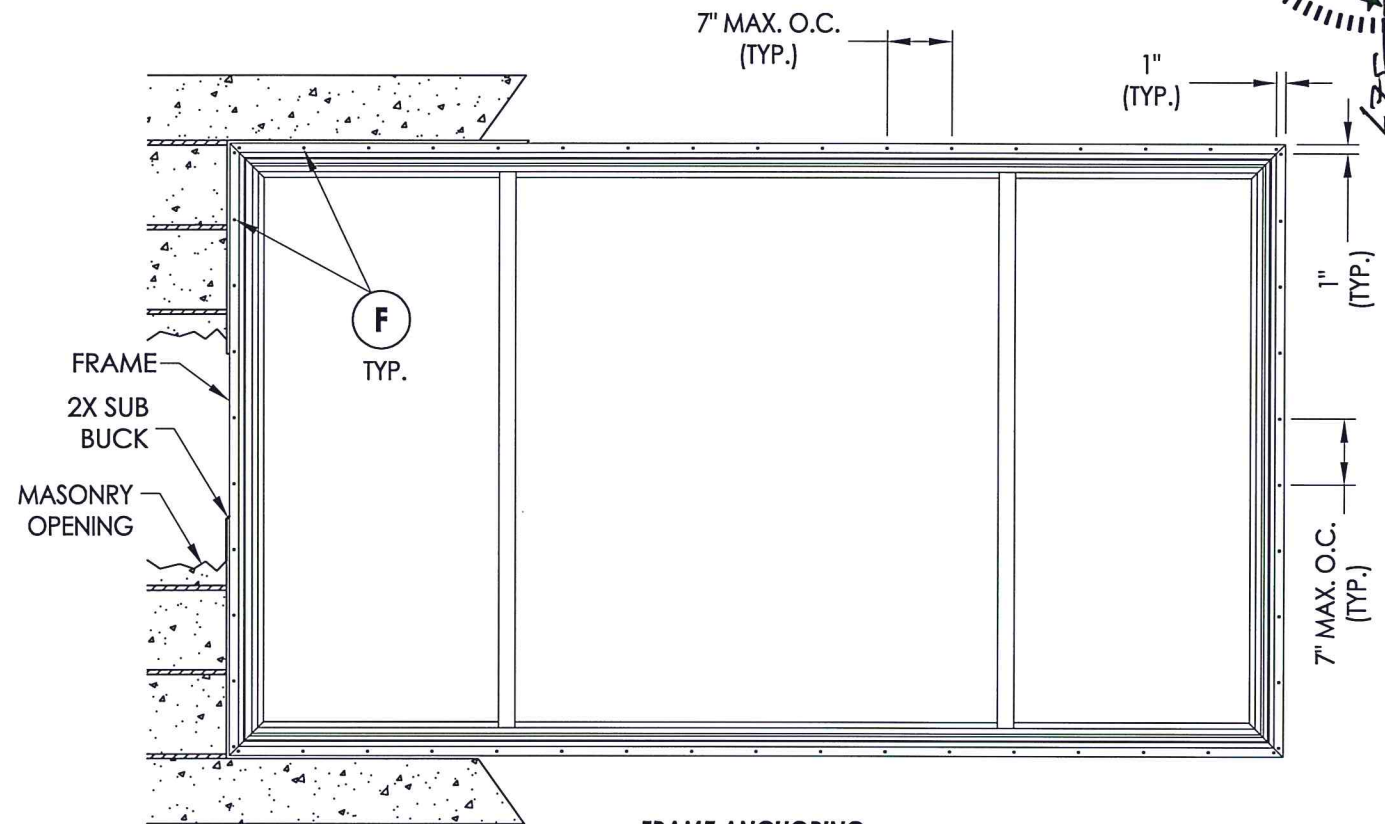
FRAME ANCHORING 2X Buck Masonry Construction
