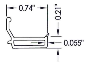
3 GLAZING BEAD
